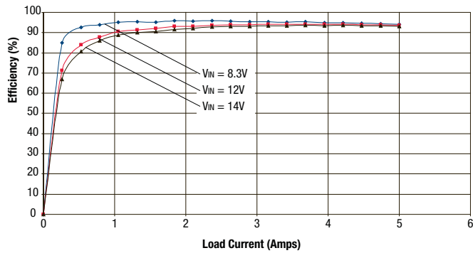
OKY-T/5-D12 Efficiency vs. Line Voltage and Load Current @ 25°C (Vout = 5V)
